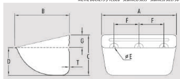
METAL BUCKETS (Pressed - Seamless steel - Stainless steel 304)
