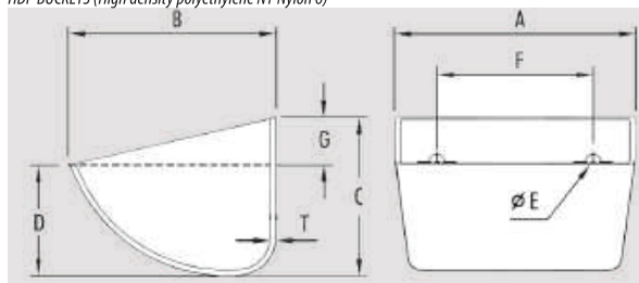
HDP BUCKETS (High density polyethylene NY Nylon 6)
